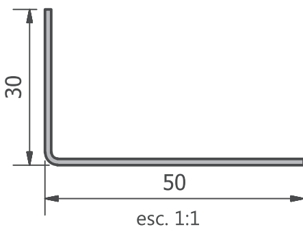
T21 - Cantoneira dobrada
