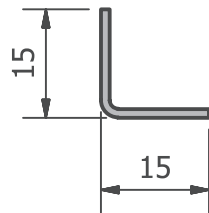
T14 - Cantoneira dobrada
